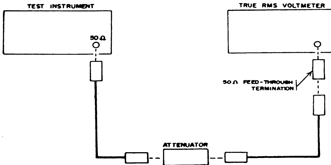
Figure 3. Output attenuator - equipment setup.
